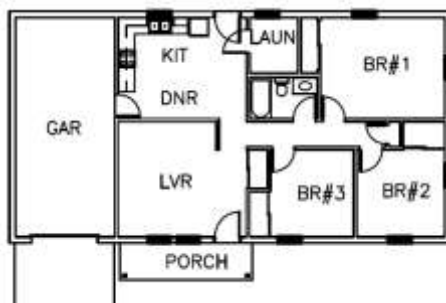
Three-Bedroom Floor Plan
